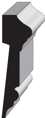
WM77 11/16 x 2-1/4
