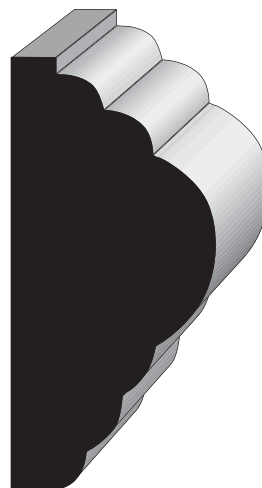
WM303 1-1/16 x 2-1/4
